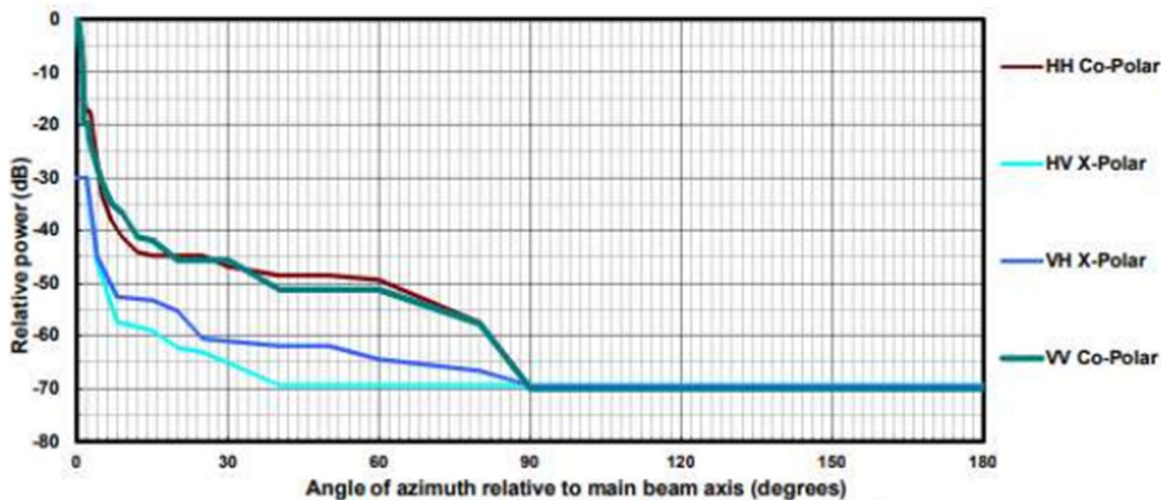
Angle of azimuth relative to main beam axis (degrees)
